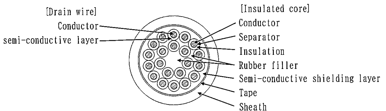
Fig. 9 Cable cross section
