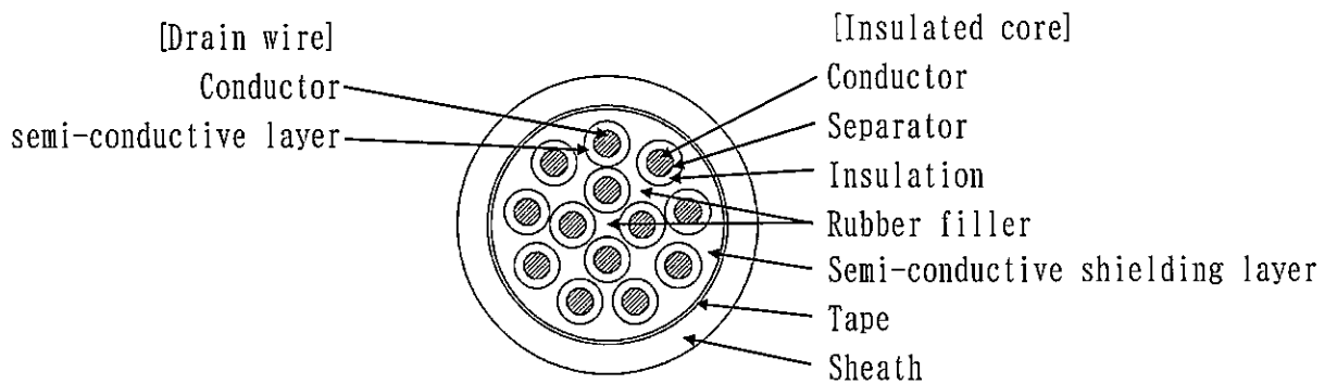
Fig. 5 Cable cross section
