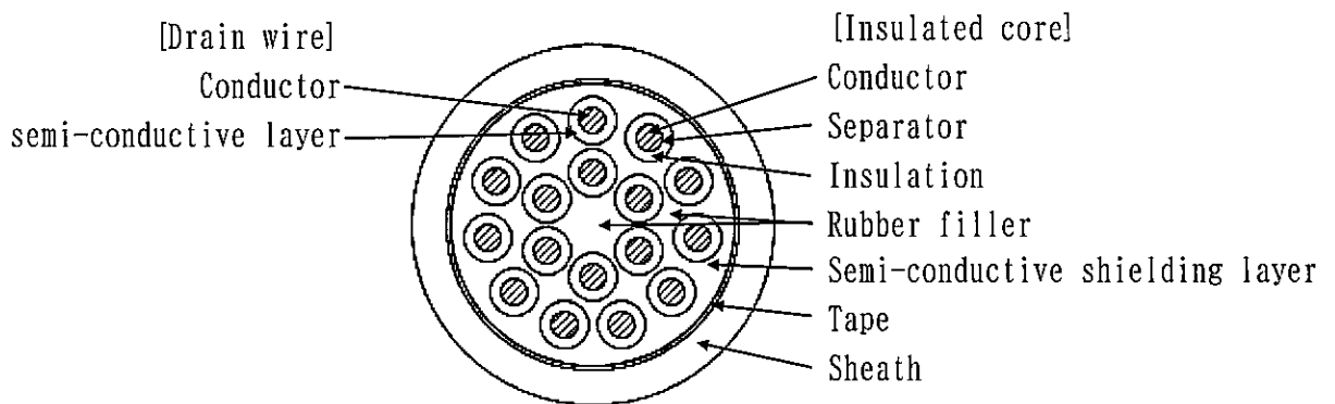
Fig.7 Cable cross section
